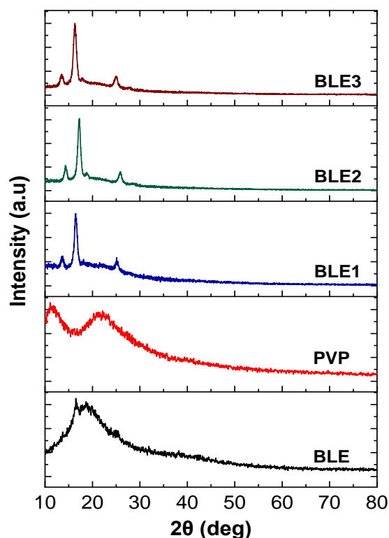
Figure 7. XRD patterns of BLE, PVP BLE1, BLE2, dan BLE3
