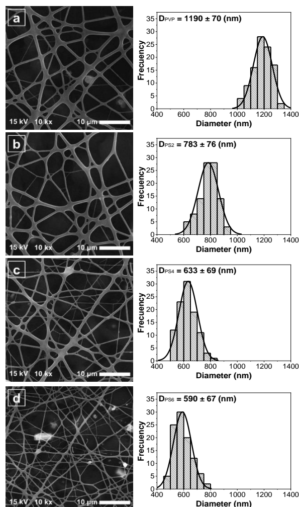
Figure 3. The Morphology and Diameter Distribution nanofibrous of (a) PVP, (b) BLE1, (c) BLE2, dan (d) BLE3.
